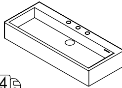
SINK - 5103 36 x 15 x 6 h GLOSS WHITE (G) --- $1080 MATTE WHITE (M) --- $1080 00, 01, 02, 03 Drain options: 7100-12, 7100-16OF, 7100-13OF
