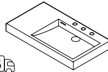
SINK - 5101RH 32 x 18 x 3 h GLOSS WHITE (G) --- $980 MATTE WHITE (M) --- $980 00, 01, 02, 03 Drain options: 7100-12, 7100-160F, 7100-130F
