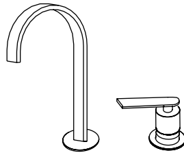
13011L SPOUT: 8 1/4 H: 14 1/2 FAUCET w/drain - Flow rate: 1.2 GPM POLISHED CHROME (CR)--- $650 C: $85
