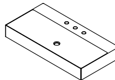
SINK - 5160 39 1/2 x 20 x 4 h GLOSS WHITE (G) --- $1030 MATTE WHITE (M) --- $1030 00, 01, 02, 03 Drain options: 7100-180F No overflow
