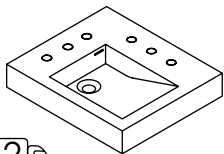
SINK - 5110 22 x 19 x 4 h GLOSS WHITE (G) --- $850 MATTE WHITE (M) --- $850 00, 01, 02, 03 mark in specs Drain options: 7100-12, 7100-16OF, 7100-13OF
