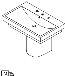
3 28 x 18 x 16 h 4271 lavatory $580 4207 shroud $150 white porcelain (001) 00, 01, 02, 03 Drain options: 7100-12, 7100-16OF, 7100-13OF
