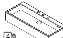
4 36 x 15 x 6 h 5103 lavatory $890 gloss white solid surface (001G) matte white solid surface (001M) 00, 01, 02, 03 Drain options: 7100-12, 7100-16OF, 7100-13OF
