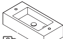
3 28 x 13 x 6 h 5099 lavatory $810 white porcelain (001) 00, 01L, 01R Drain options: 7100-12, 7100-16OF, 7100-13OF
