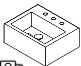
2 15 x 11 1/2 x 6 h 5088 lavatory $340 white porcelain (001) 00, 01, 02, 03 Drain options: 7100-12, 7100-16OF, 7100-13OF
