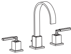
SPOUT: 6 SPREAD: 4-11 3/4 H: 10 1403 faucet w/drain Flow rate: 2.1 GPM (60 PSI) $790 CR $950 NI C $100
