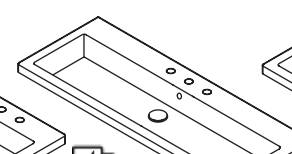
4 48 x 18 x 5 h 5215 lavatory $1,190 white porcelain (001) 00, 01, 02, 03, or per specs Drain options: 7100-12, 7100-16OF, 7100-13OF
