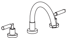
SPOUT: 9 1/2 H: 8 3/8 1593 tub filler Flow rate: 10.2 GPM (60 PSI) $690 C $150
