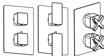
W: 5 1/8 H: 7 1/4 1844 1844L 1844X thermostat w/OFF and 2-way diverter Flow rate: 7.4 GPM (43.5 PSI) $990 A $590 B $400 D $100 CT $155 EX $155
