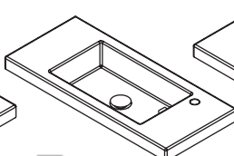
3 32 x 14 x 6 h 5273 lavatory $680 white porcelain (001) 00, 01 Drain options: 7100-12, 7100-16OF, 7100-13OF
