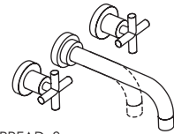
SPREAD: 8 1585 faucet SPOUT: 6 3/8 1585L faucet SPOUT: 9 7/8 Flow rate: 1 GPM $610 A $365 B $245 C $100 EX $100
