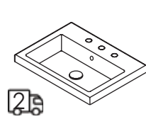
2 24 x 18 x 5 h 5211 lavatory $490 white porcelain (001) 00, 01, 02, 03 Drain options: 7100-12, 7100-16OF, 7100-13OF
