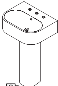
2 20 x 16 x 33 h 2962 lavatory $410 4231 pedestal $175 white porcelain (001) 01, 02, 03 Drain options: 7100-12
