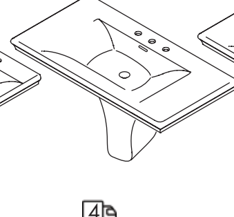
3 28 x 21 x 34 h GL28 lavatory $960 GL31 pedestal $500 white porcelain (001) 01, 02, 03 Drain options: 7100-12
