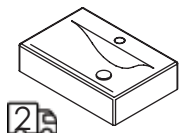
2 24 x 13 x 6 h 5461 lavatory $540 white porcelain (001) 01, 02, 03 Drain options: 7100-13
