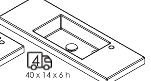
4 40 x 14 x 6 h 5274 lavatory $890 white porcelain (001) 00, 01 Drain options: 7100-12, 7100-16OF, 7100-13OF
