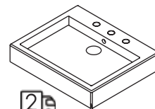
2 22 x 19 x 4 h 5030FB lavatory $490 white porcelain (001) 00, 01, 02, 03 Drain options: 7100-12, 7100-16OF, 7100-13OF
