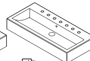
4 40 x 19 x 6 h 5460 lavatory $960 white porcelain (001) 00, 01, 02, 03, or per specs Drain options: 7100-12, 7100-16OF, 7100-13OF
