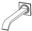
SPOUT: 7 3/8 W: 2 1/2 H: 2 1/2 1455 spout $260 CR $315 NI
