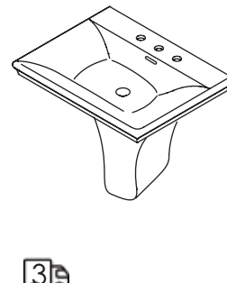
3 28 x 21 x 22 h GL28 lavatory $960 GL07 shroud $430 white porcelain (001) 01, 02, 03 Drain options: 7100-12
