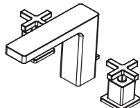
SPOUT: 6 H: 5 1/8 1803X faucet w/drain Flow rate: 1.3 GPM $790 C $100
