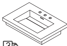
3 30 x 21 x 6 1/2 h H262T lavatory $880 gloss white solid surface (001G) matte white solid surface (001M) 00, 01, 02, 03 Drain options: 7100-18OF
