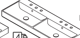
4 48 x 18 x 7 h 5234 lavatory $1,190 white porcelain (001) 00, 01, 02, 03 Drain options: 7100-12, 7100-16OF, 7100-13OF
