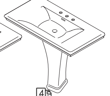
4 40 x 21 x 22 h GL40 lavatory $1,550 GL07 shroud $430 white porcelain (001) 01, 02, 03 Drain options: 7100-12
