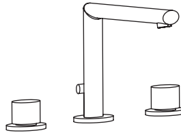
SPOUT: 5 3/8 SPREAD: 6-11 3/4 H: 7 1/4 0603 faucet w/drain Flow rate: 2.2 GPM (60 PSI) $790 C $120
