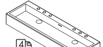
4 48 x 15 x 6 h 5104 lavatory $1,050 gloss white solid surface (001G) matte white solid surface (001M) 00, 01, 02, 03 Drain options: 7100-12, 7100-16OF, 7100-13OF
