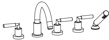
SPOUT: 9 1/2 H: 8 3/8 1532 tub filler Flow rate: 6.4 GPM (60 PSI) $1,150 C $150 D $100
